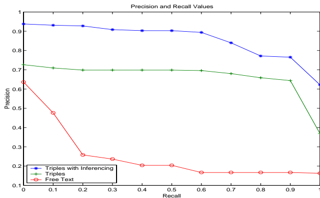
Figure 7: Precision and Recall Values
