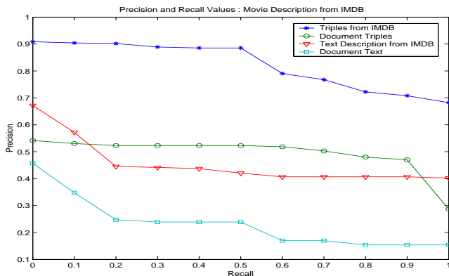
Figure 8: Precision and Recall Values - Enhanced Triples from IMDB
