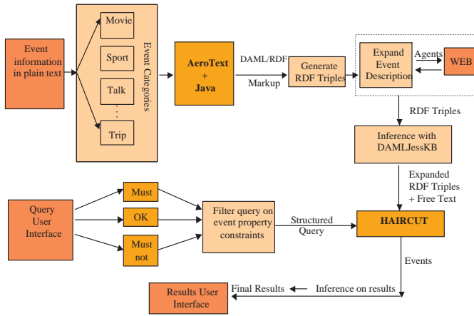
Figure 4: OWLIR Process Flow
