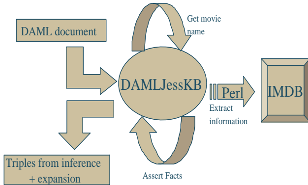
Figure 5: Information from IMDB Site
