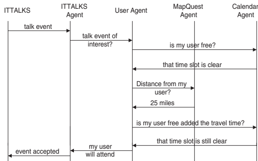
Fig. 4. Interactions between the various agents described in the ITTALKS/Agent scenario
