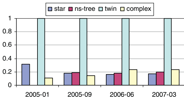
Fig. 9. The evolution of density distribution of components (grouped by structural patterns).
