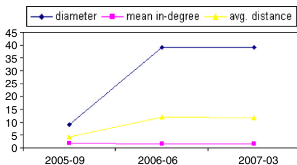
Fig. 11. The evolution of diameter, mean in-degree, and average distance of the largest component.
