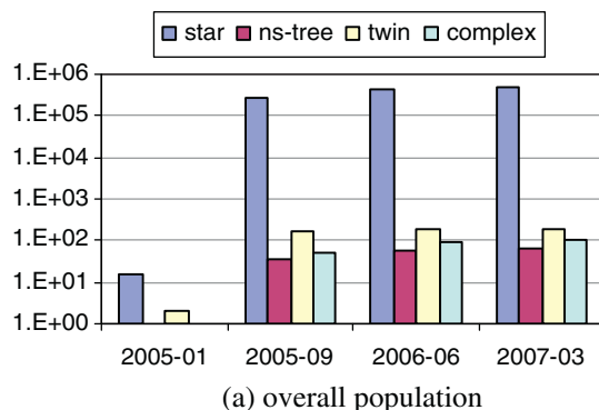
Fig. 7. The evolution of population and average size of components (grouped by structural patterns).
