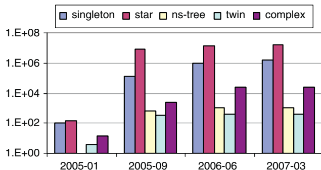
Fig. 6. The evolution of node distribution (grouped by structural patterns).
