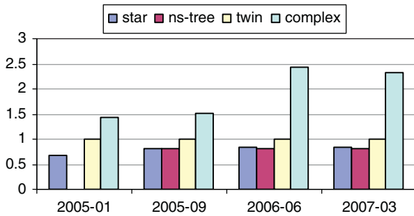
Fig. 8. The evolution of average in-degree distribution of components (grouped by structural patterns).
