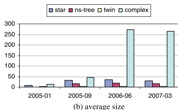
Fig. 7. The evolution of population and average size of components (grouped by structural patterns).
