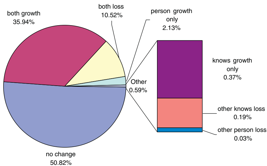
Fig. 2. Types of changes to FOAF documents.
