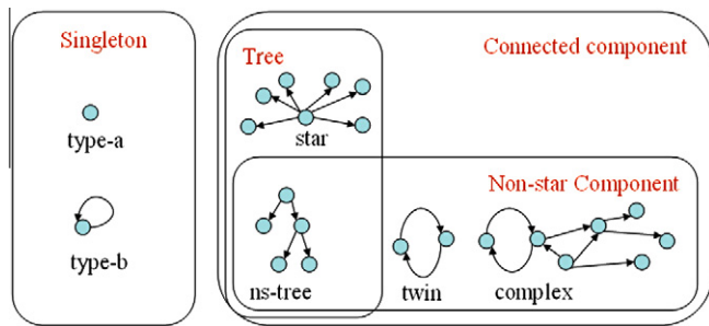
Fig. 5. Typical structural patterns of FOAF networks.
