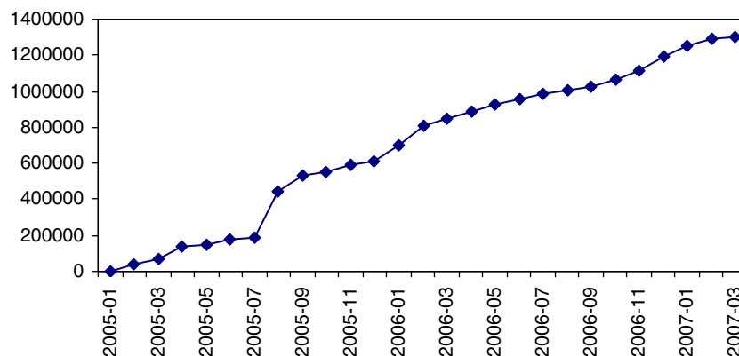
Fig. 3. The trend of accumulative FOAF document revisions.
