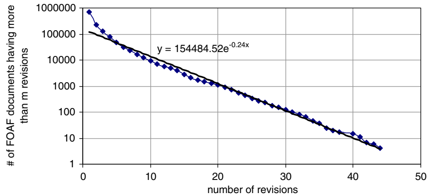
Fig. 1. The distribution of accumulative frequency of FOAF document revisions.
