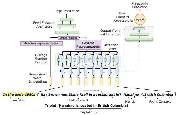
Figure 3: The joint learning architecture for training KGE and entity typing takes in both factual triplets and context information for an entity. Parameters of the architecture are trained to learn both the factual information as well as the corresponding entity types.
