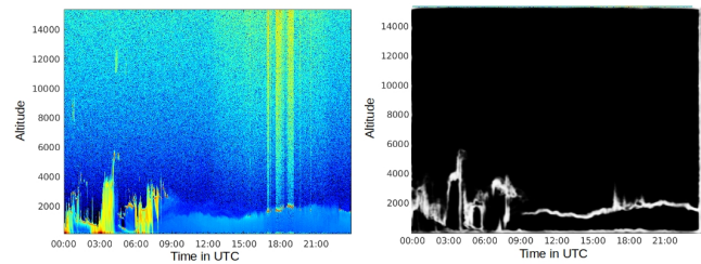
Figure 1: Lufft-CHM15K - UMBC - (left) 24 Hour LIDAR Backscatter Profiles and (right) Backscatter Image Boundary Detection (ML-PBLH)- 12/1/2016.
