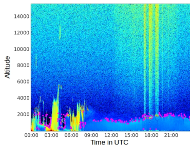
Figure 2: Lufft-CHM15K - UMBC - 24 Hour LIDAR Backscatter Profiles and PBLH Points Generated from our Backscatter Image Boundary Detection (ML-PBLH) - 12/1/2016.
