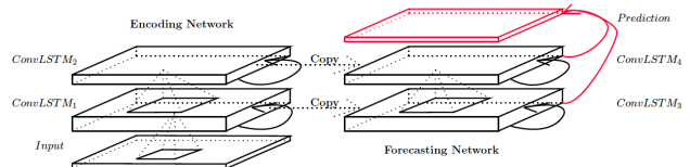
Figure 3: ConvLSTM Architecture (Shi et al.)
