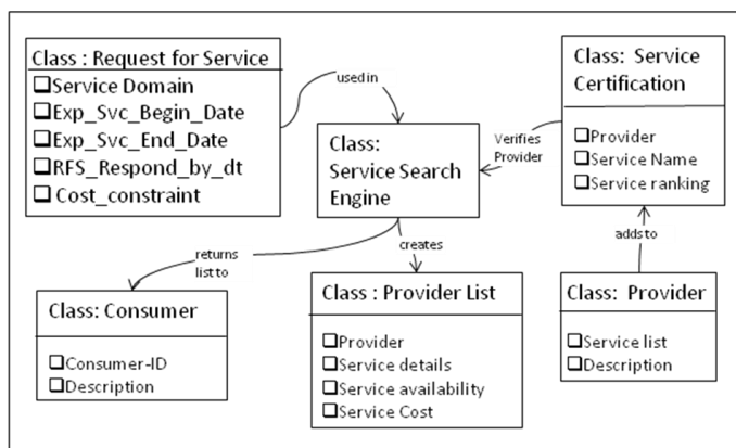
Figure 4: Ontology for service discovery phase uses the RFS class to search for providers and generate a Provider list
