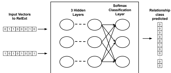
Fig. 3: Relationship Extractor - A Feed Forward Neural Network
